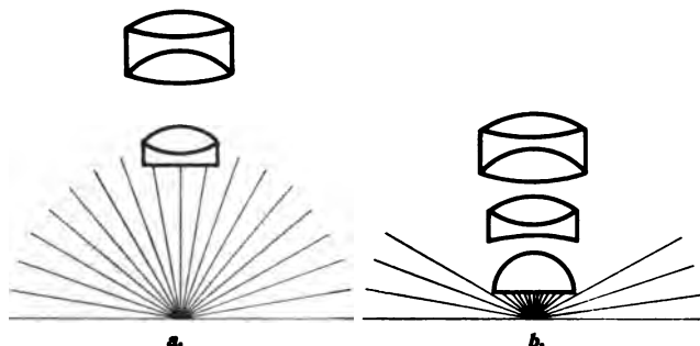
Diagrammatic representation of light transmitted by objectives of low ( a ) and high ( b ) angular aperture.
